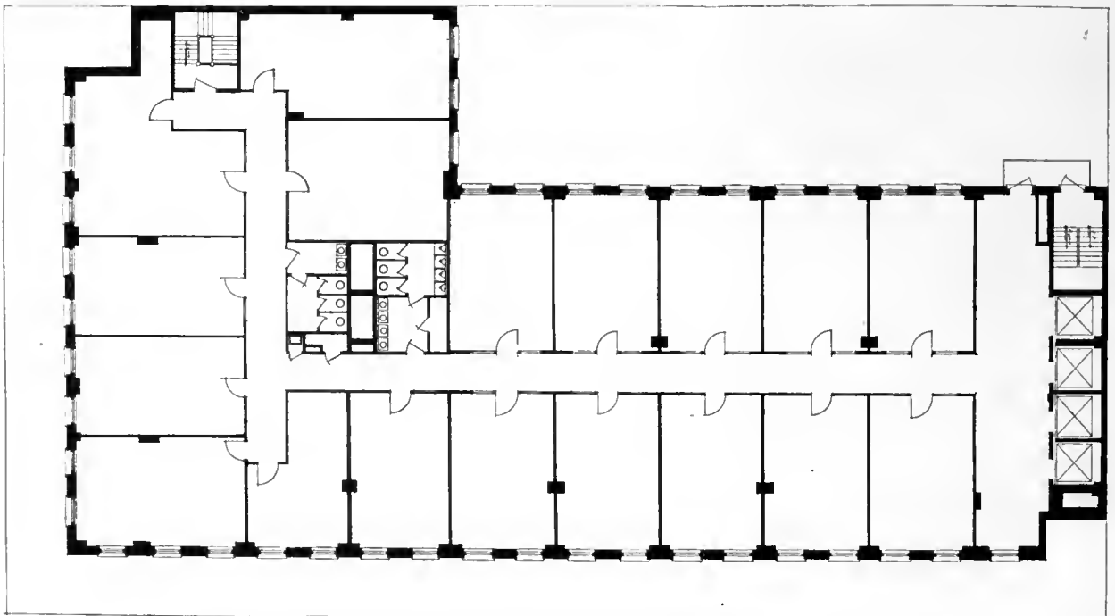
FIRST AND SECOND PENT HOUSE FLOOR PLANS BUILDING FOR S. W. STRAUS & CO., FIFTH AVENUE AT 46TH STREET, NEW YORK WARREN & WETMORE, ARCHITECTS
